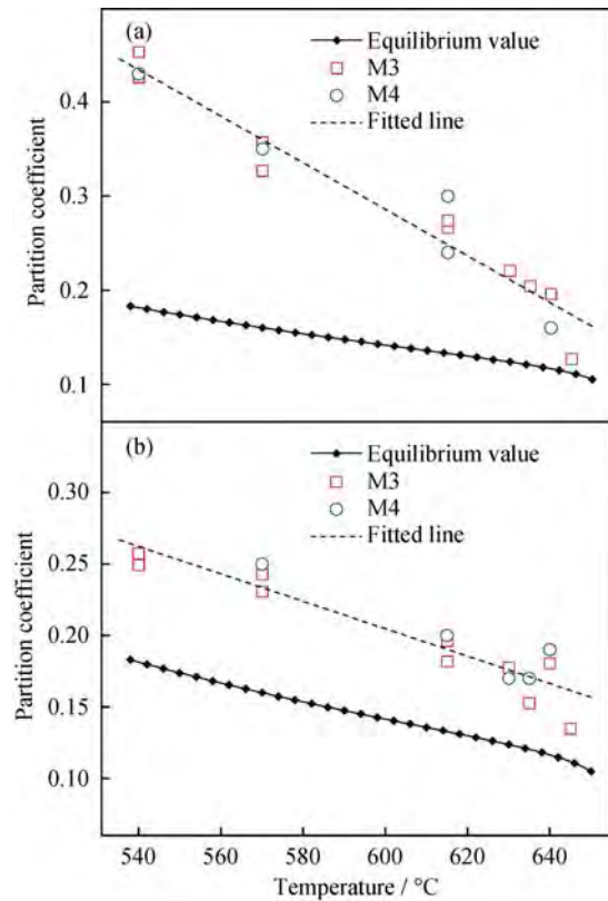
Fig. 6. Experimental and equilibrium values of k_0 at different cooling rates: (a) 0.5 K·min -1 ; (b) 5 K·min -1 .
