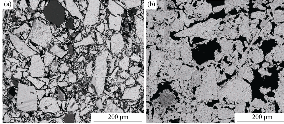
Fig. 5. SEM images of the vanadium titano-magnetite before gas-based reduction: (a) raw samples; (b) samples after pre-oxidation.
