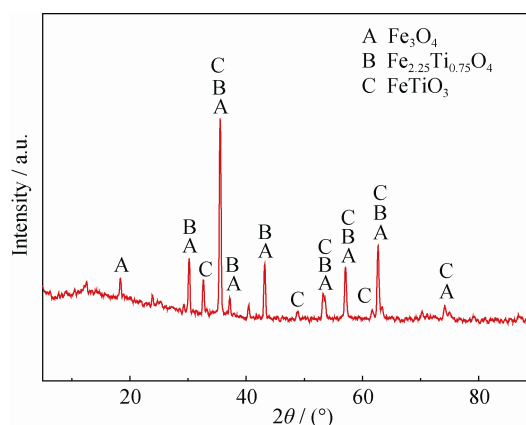
Fig. 1. XRD pattern of vanadium-bearing titanomagnetite used in the experiments.
