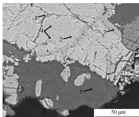
Fig. 2. SEM image of vanadium-bearing titanomagnetite.
