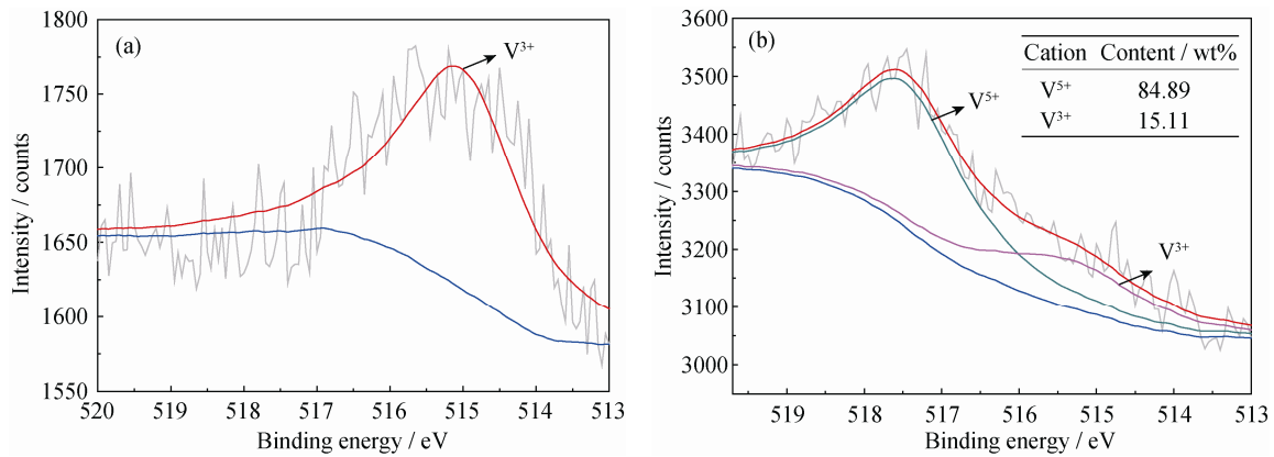
Fig. 5. XPS spectra of V2p_{3/2} of the vanadium-bearing titanomagnetite (a) and the product roasted at 1200^{\circ}\text{C} (b).
