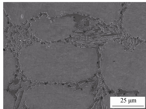
Fig. 2. SEM micrograph of the as-cast HK40 steel.
