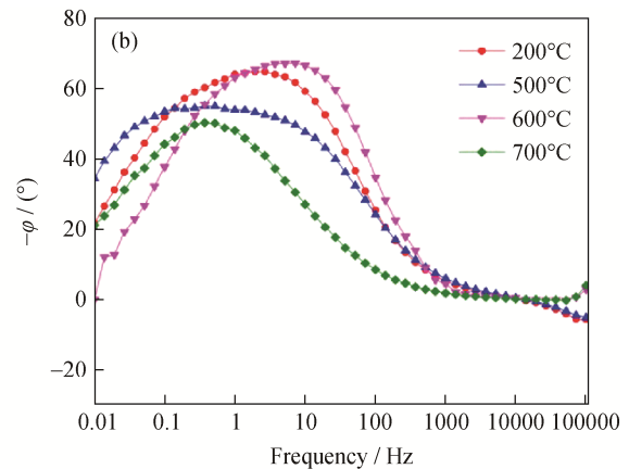
Fig. 7. Bode plots of the examined samples tempered at various temperatures ( |Z| is the modulus of impedance; \varphi is the phase angle): (a) modulus of impedance–frequency; (b) phase angle–frequency.
