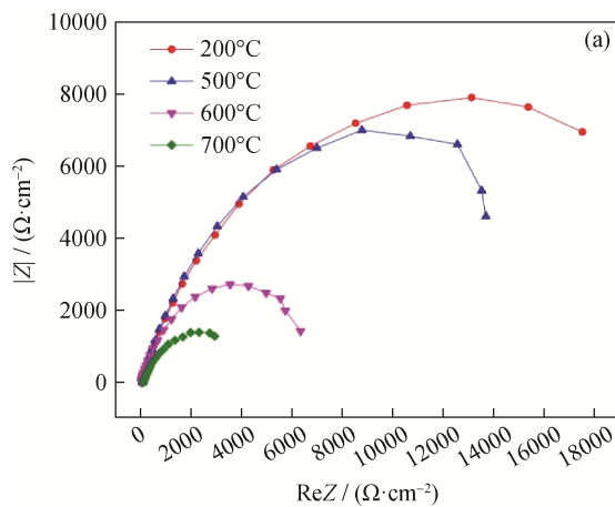
Fig. 6. Nyquist plots (a) and the equivalent electrical circuit of the examined samples (b).
