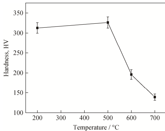
Fig. 2. Trend of hardness with different tempering temperatures.
