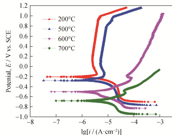
Fig. 5. Polarization curves of the examined samples with different tempering temperatures (the curves were recorded with the samples immersed in electrolyte solution).
