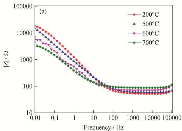
Fig. 7. Bode plots of the examined samples tempered at various temperatures ( |Z| is the modulus of impedance; \varphi is the phase angle): (a) modulus of impedance–frequency; (b) phase angle–frequency.
