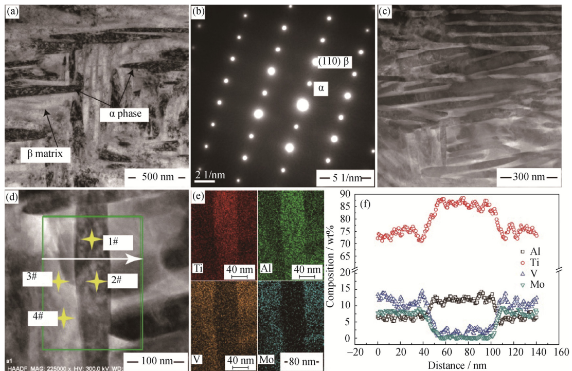
Fig. 9. Microscopic analysis of the Ti64–6Mo alloy after aging at 600°C: (a) bright-field morphology; (b) SAED pattern with [111] \beta zone axis; (c and d) HAADF–STEM images showing the \alpha phase; (e) the EDS mapping of Mo, V, Al, and Ti atoms; (f) the composition profiles along the arrows shown in (d).
