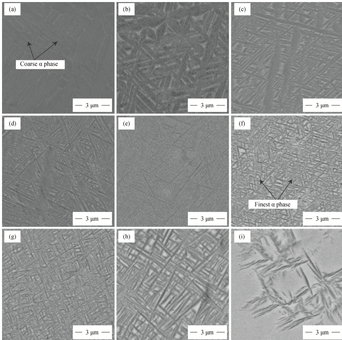
Fig. 5. Backscattered-electron images of aged (600°C for 6 h) Ti64– x Mo alloys obtained from the Ti6Al4V–Ti6Al4V20Mo diffusion couple: (a) Ti6Al4V; (b) Ti6Al4V1Mo; (c) Ti6Al4V2Mo; (d) Ti6Al4V4Mo; (e) Ti6Al4V5Mo; (f) Ti6Al4V6Mo; (g) Ti6Al4V8Mo; (h) Ti6Al4V11Mo; (i) Ti6Al4V15Mo.
