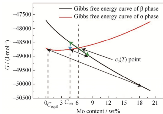
Fig. 15. Gibbs free-energy curves for \alpha and \beta phases of Ti64– x Mo alloy at 600°C (the green arrow indicates component fluctuations; the blue arrow represents component fluctuations causing the \alpha -phase free energy to be lower than the \beta -phase free-energy).
