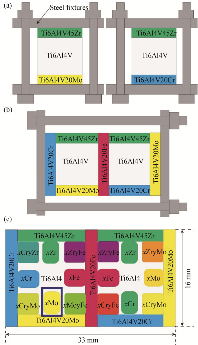
Fig. 1. Preparation process of diffusion multiple Ti6Al4V-Ti6Al4V45Zr-Ti6Al4V20Mo-Ti6Al4V20Fe-Ti6Al4V20Cr: (a) preparation of two sandwich diffusion couples with steel fixtures; (b) preparation of the diffusion multiple using a steel fixture; (c) cross-sectional schematics of the diffusion multiple.
