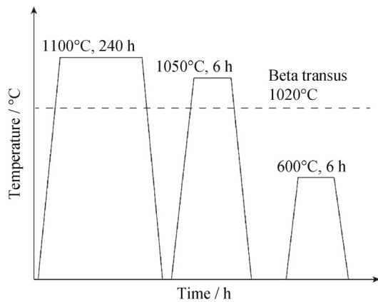
Fig. 2. Heat-treatment flow chart for the Ti6Al4V-Ti6Al4V45Zr-Ti6Al4V20Mo-Ti6Al4V20Fe-Ti6Al4V20Cr diffusion multiple.
