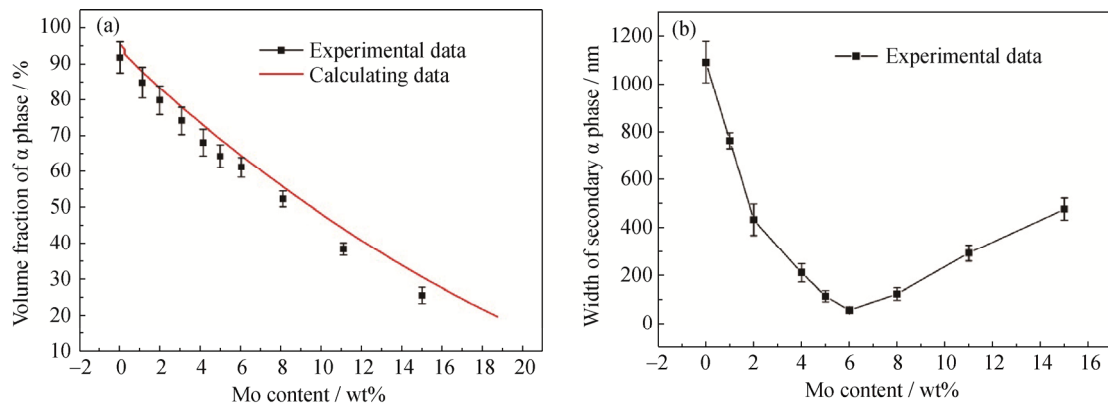
Fig. 6. Volume fraction of the α phase (calculation and experimental results) varies with the Mo content in the sample aged at 600°C (a) and the width of the α phase varies with the Mo content in the sample aged at 600°C (b).
