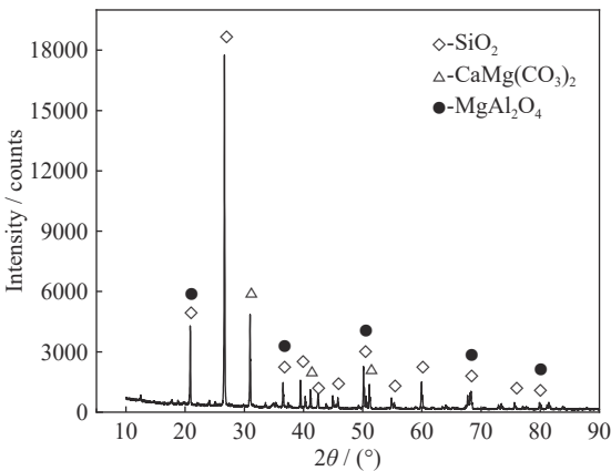
Fig. 1. XRD pattern of the low-grade Co ore.
