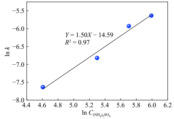
Fig. 17. Fitting relationship between \ln k and \ln C_{(\text{NH}_4)_2\text{SO}_4} .
