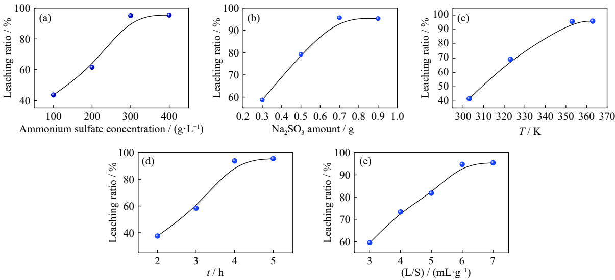
Fig. 5. Effect of (NH 4 ) 2 SO 4 concentration (a), Na 2 SO 3 amount (b), leaching temperature T (c), leaching time t (d), and liquid–solid ratio (e) on the Co leaching ratio.
