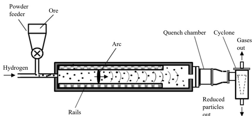
Fig. 8. Principles of design of rail reactor. Adapted from Ref. [66].
