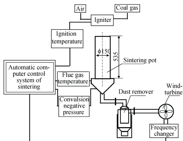
Fig. 2. Sketch of the sinter pot system.
