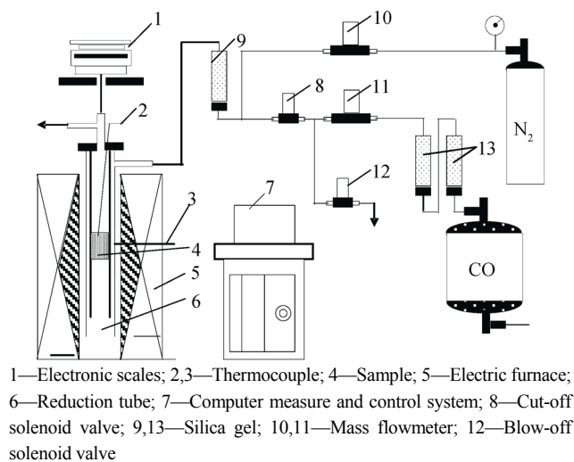
Fig. 3. Equipment used in low-temperature reduction disintegration.
