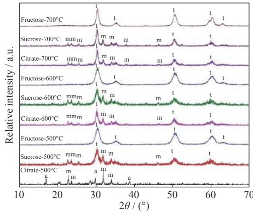
Fig. 3. X-ray diffraction patterns of the calcined powders (t: tetragonal zirconia; m: monoclinic zirconia; a: ammonium nitrate).
